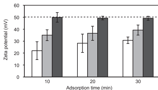
Fig. 6. The influence of (□) malic acid, (▤) malonic acid, and (■) acetic acid adsorption on TiO 2 zeta potential in the absence of light. (—) The average zeta potential of pure TiO 2 without any organics present. Initial experimental conditions: TiO 2 concentration: 0.2 g L -1 ; organic loading: 2000 μg C; pH: 3 ± 0.05.
