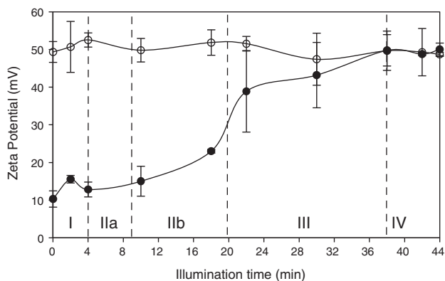
Fig. 5. Change in the zeta potential of (○) illuminated aqueous TiO 2 suspension and (●) illuminated reaction mixture/TiO 2 suspension.
