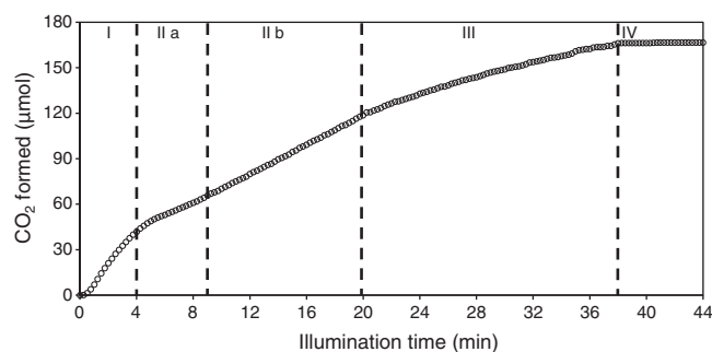
Fig. 1. Photomineralization profile of malic acid in a TiO 2 suspension using a spiral, slurry-type reactor. Initial experimental conditions: TiO 2 concentration: 0.2 g L -1 ; malic acid: 2000 μg C; pH: 3 ± 0.05.
